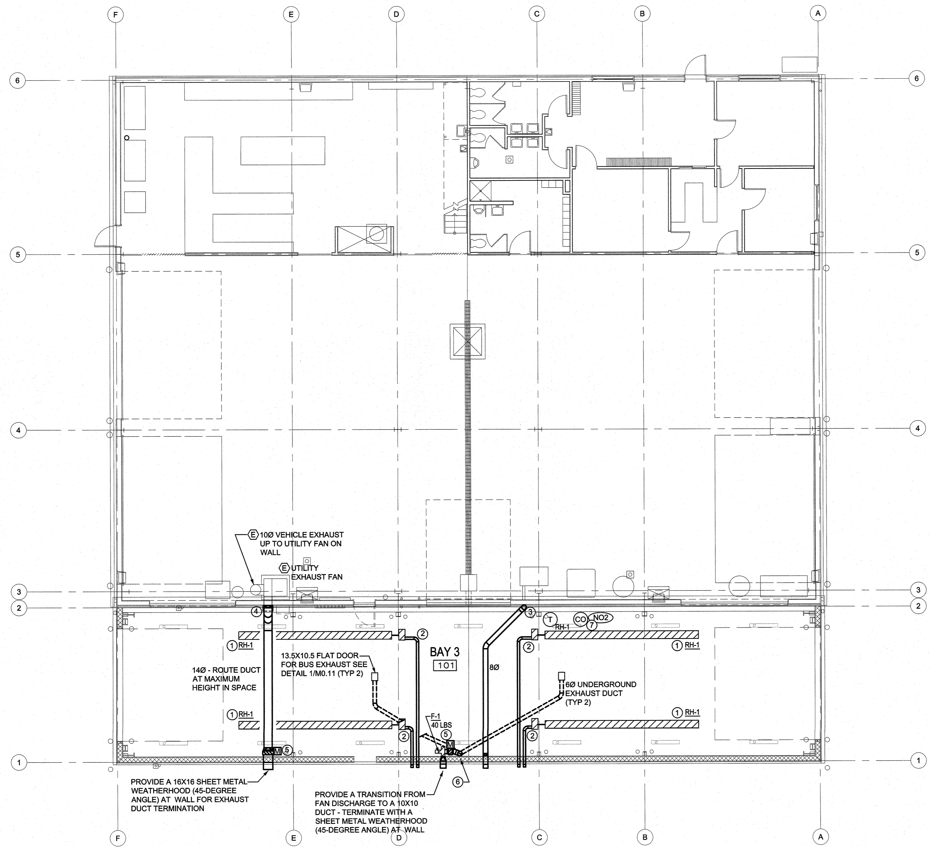
1 SHOP BUILDING FLOOR PLAN
