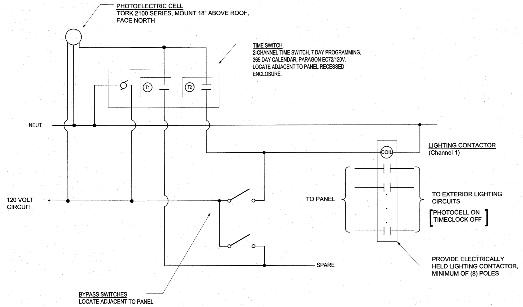
1 DETAIL - LIGHTING CONTROL NO SCALE
