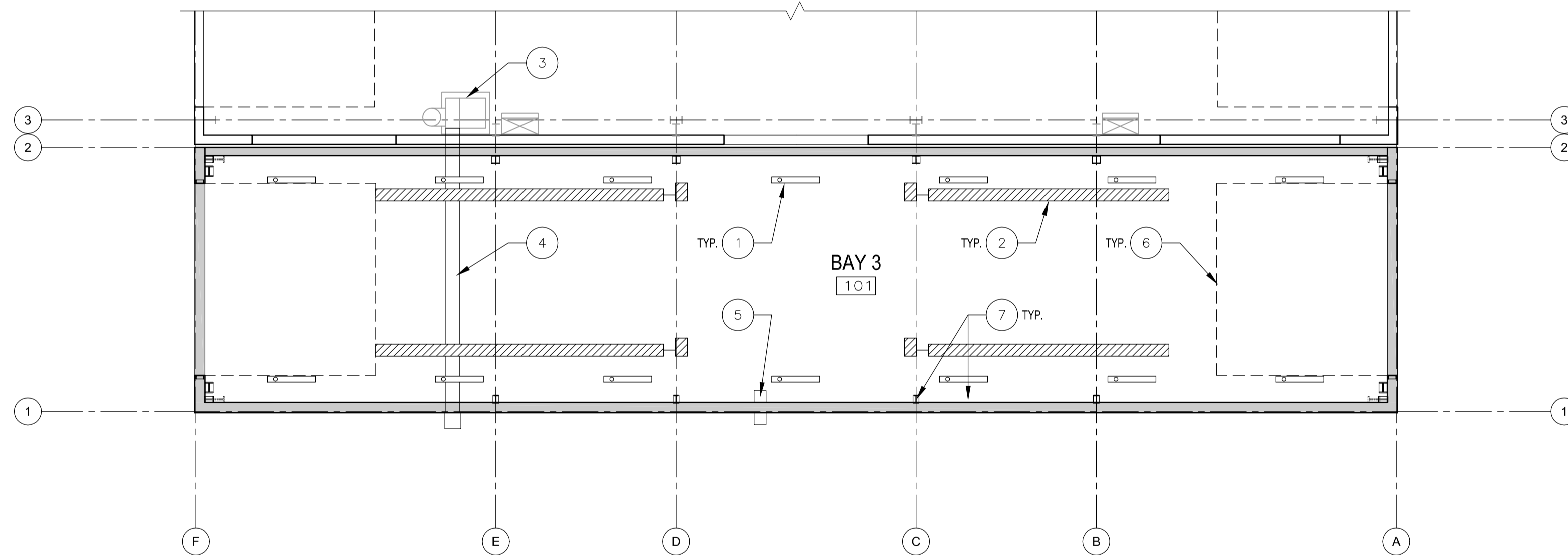
1 SHOP BUILDING REFLECTED CEILING PLAN
